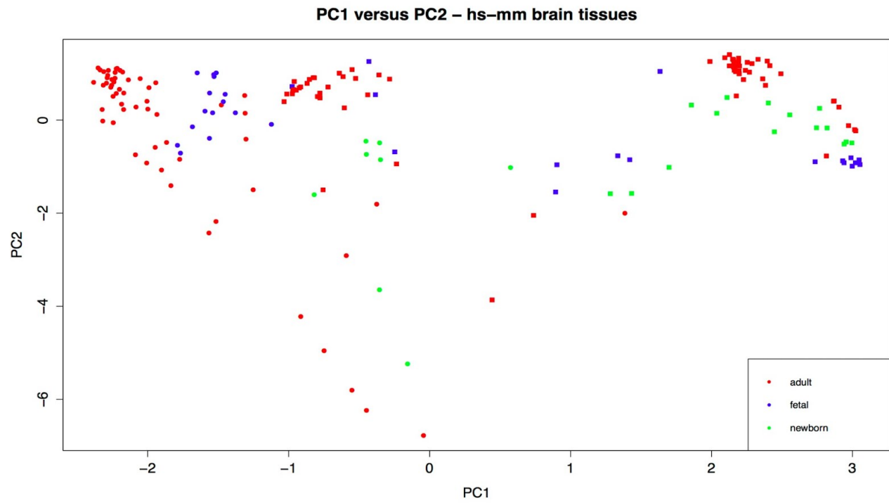
Fig. * Human brain tissues cluster based on the development stage, but the same pattern can't be seen in mouse
