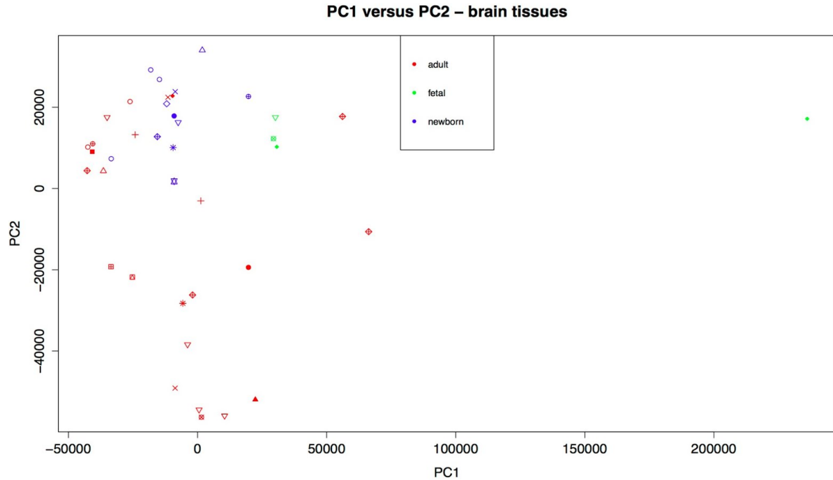
Fig1. Initial exploration of expression pattern diversity in F5 encyclopedia using PCA. Human brain tissues stand out as showing unexpected differential regulation into foetal, newborn and adult samples.
