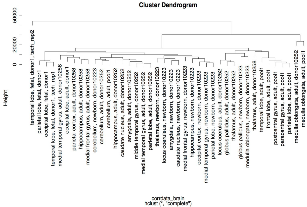
Fig. * Human brain tissues clusters based on euclidian distances between expression levels in samples.
