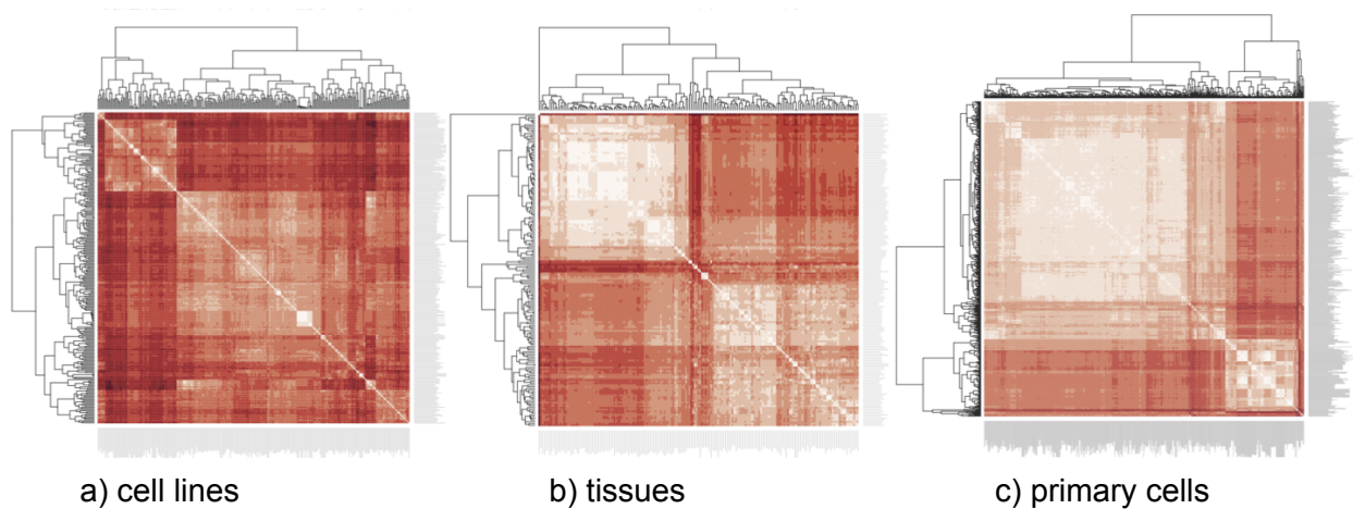
Fig2. Clustering of human samples subdivided into major biological classes (tissues, primary cell-lines, cancer cell-lines and time-courses)
