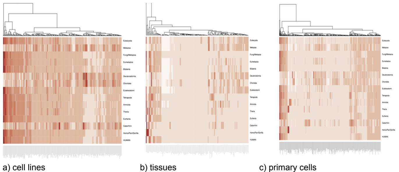
Fig9. Evolutionary history of tissues and primary cells is revealed through phylogenetically-aware expression profiling. Further evidence for expression pattern devolution in cancer cell lines. (m3_data)
