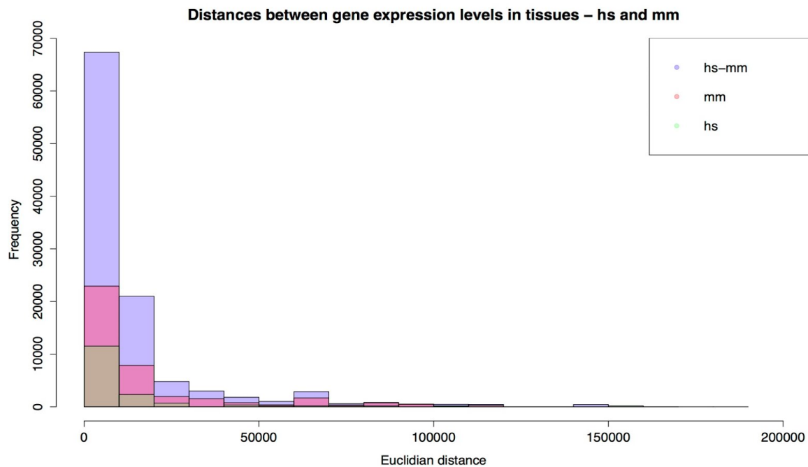
Fig. * Comparison of the expression divergense between paralogs in human, mouse and in the joint data. Euclidian distances between expression levels in paralogs are much higher inbetween the species.
