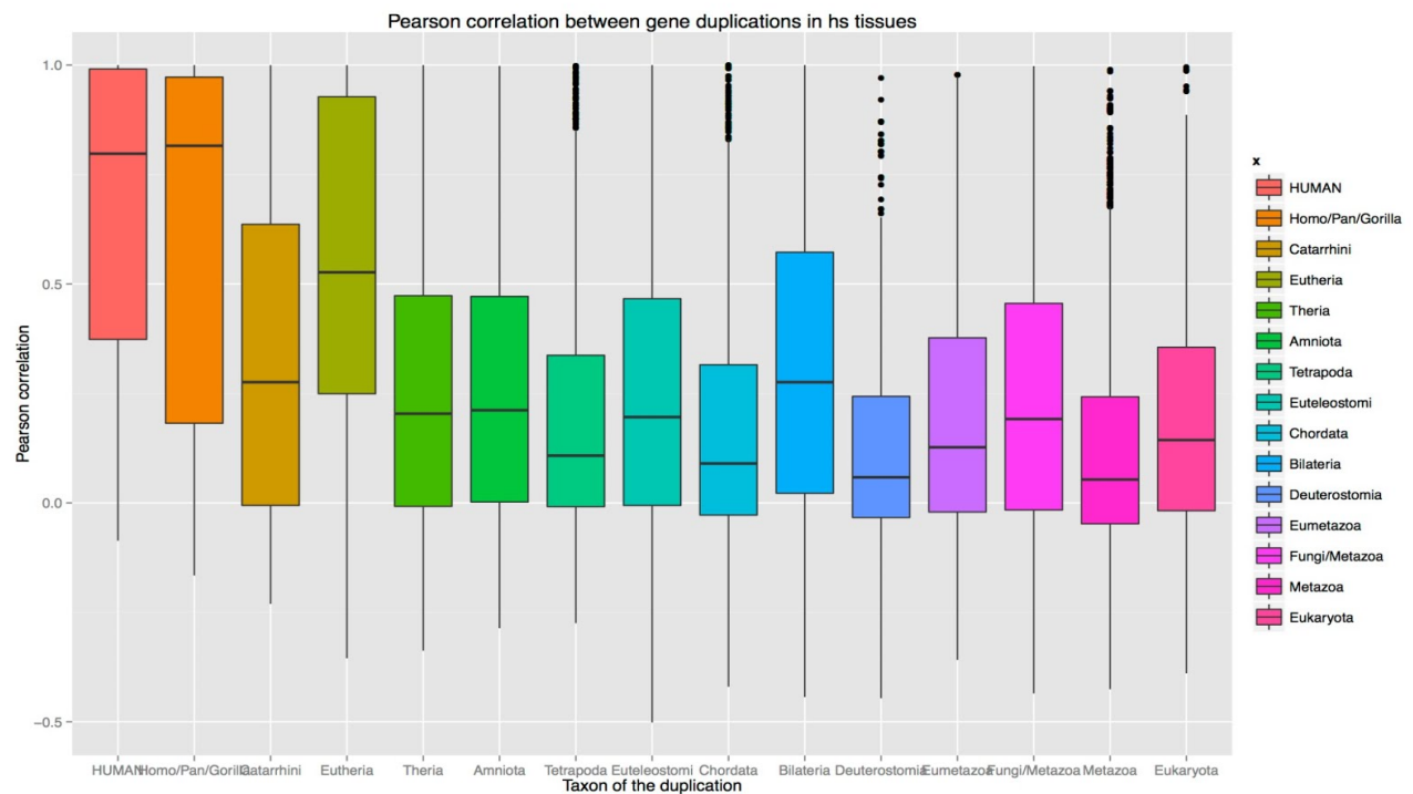
Fig6. Young genes are tissue-specific and diverge fast; old genes are housekeeping and more stable in their expression status over evolutionary time
